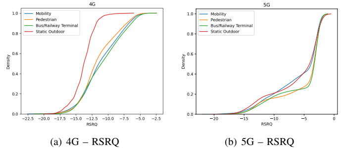
Fig. 4: 4G vs. 5G RSRQ.
