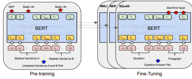
Figure 2: BERT architecture [7]
