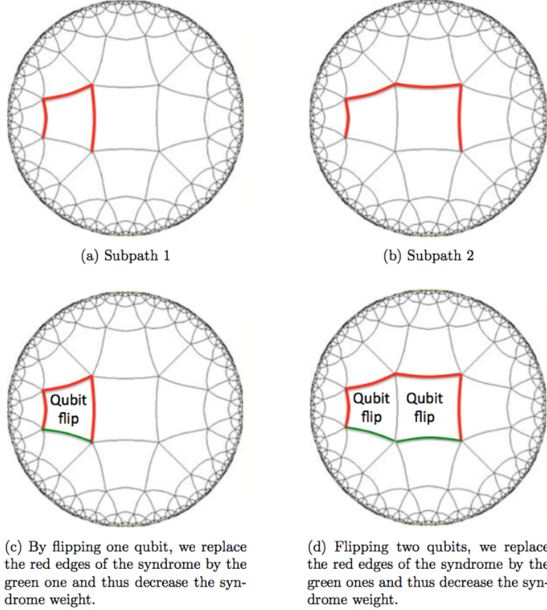
Fig. A.1. In the \{4, 5\} tessellation of hyperbolic plane, every loop of edges contains one of the two subpaths in red. These two subpaths are not minimal: they can be replaced by the shorter green ones by flipping one or two qubits. (source for image: [31])
