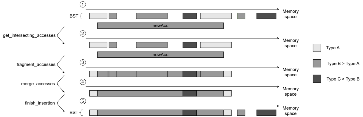
Figure 4: Illustration of the insertion of a new memory access in the BST.
