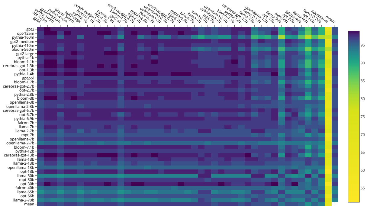
Figure 1: 5-seed averaged AUC scores for a classifier trained on text from a source model ( Side axis ) and tested on text from a target model ( Top axis ). We provide the full results table with values in Appendix A.
