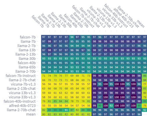
Figure 4: Conversational models cross-model detection with their foundation LLM (5-seed averaged AUCROC score).
