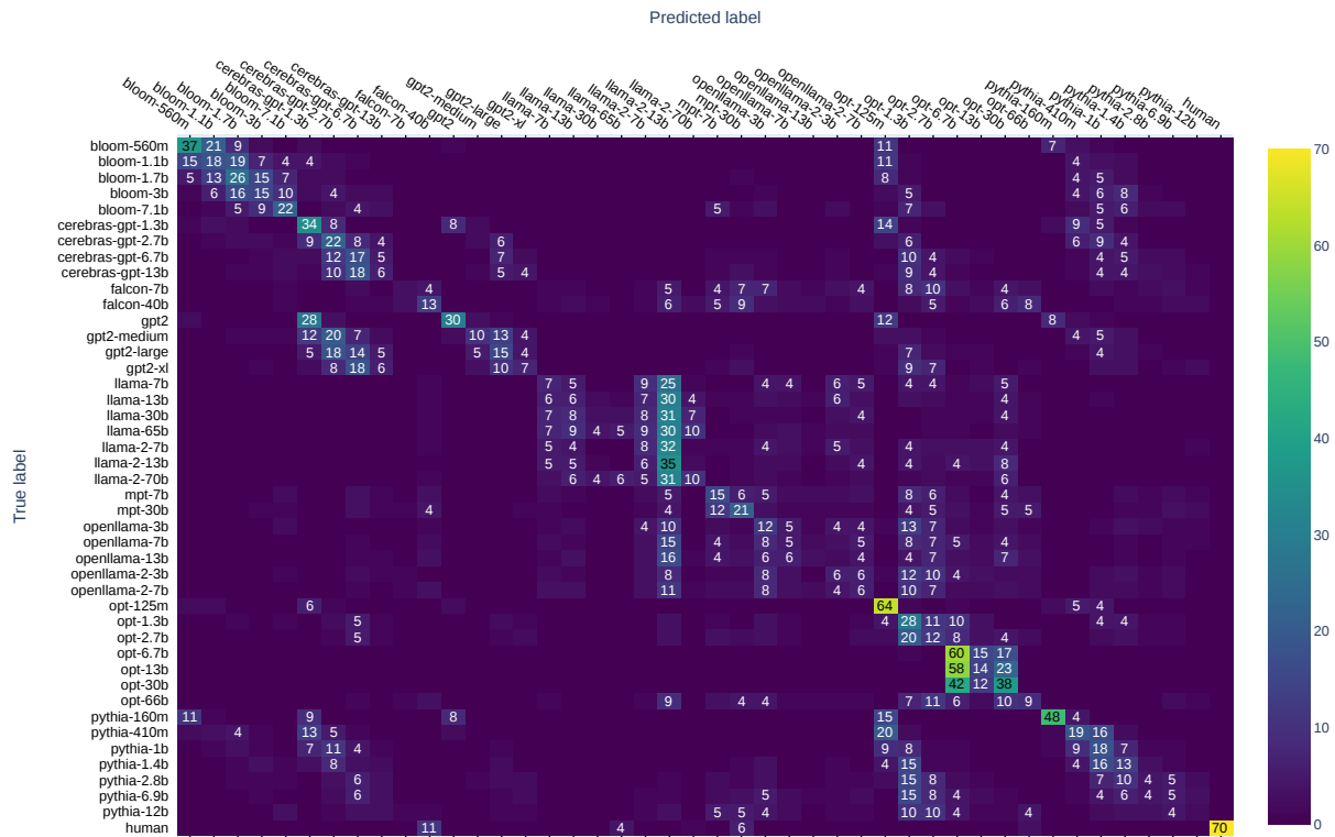
Figure 3: Normalized confusion matrix for Source Model Identification. 5-seed averaged and normalized by the predicted class support. For clarity purposes, we hide labels on values less than 4.
