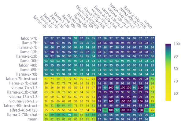
Figure 4: Conversational models cross-model detection with their foundation LLM (5-seed averaged AUCROC score).
