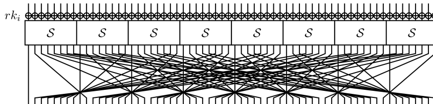
Fig. 4. FLY round function (Figure 5.2 in [36] ).
