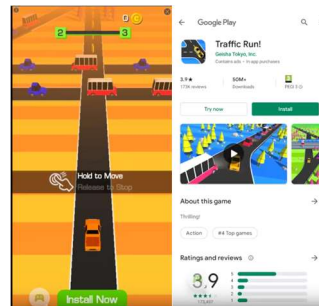
Fig. 2: Deceptive Advergame
