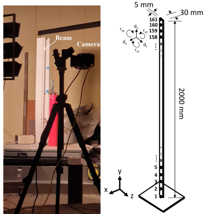
Fig. 1. Experimental setup and finite element (FE) model of cantilever beam
