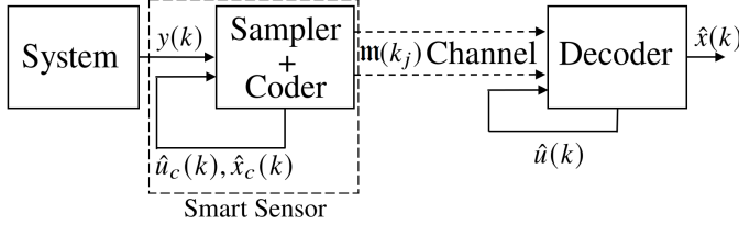
Fig. 1. Structure of setup.
