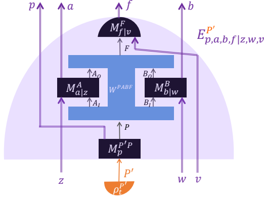
Figure 5: (P+2+F) -partite SDI-QI scenario with quantum inputs solely for Phil. The trusted quantum input (orange) \rho_t \in \mathcal{L}(\mathcal{H}^{P'}) is prepared and effectively measured by the D-POVMs (E_{p,a,b,f|z,w,v}^{P'})_{p,a,b,f} generated by Phil, Alice, Bob and Fiona's untrusted operations on the process matrix W^{PABF} .
