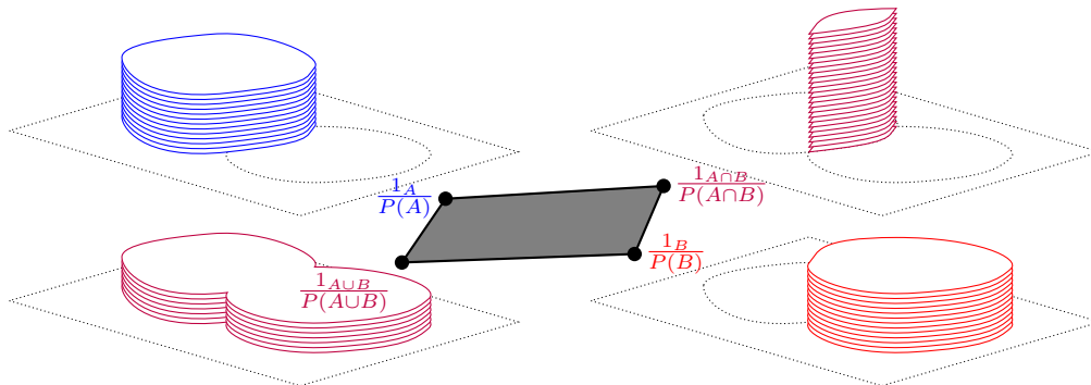
Figure 5: An example of a 2-face of the total variation unit ball \{\text{TV} \leq 1\} . Such a face has more than 3 extreme points and therefore it is not exposed by any C^1 function, by virtue of Theorem 3.8 (notice that A \cap B and A \cup B are not smooth).
