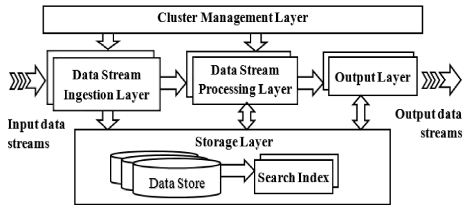
Fig. 1. Architecture of a typical data stream processing system (adapted from [21]).
