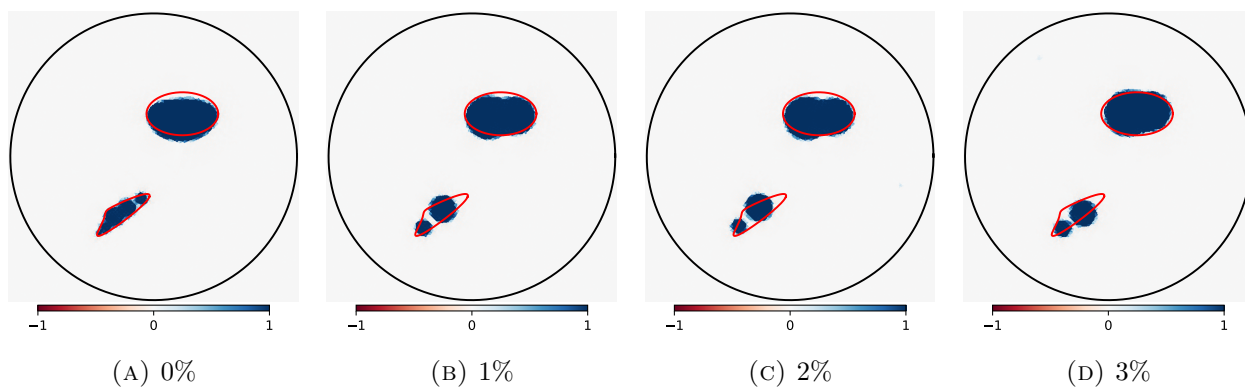
FIGURE 5.6. Reconstruction of a domain convex in one direction with noisy data ( N = 12 )
