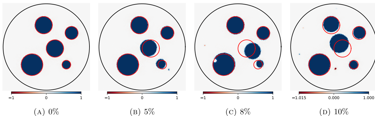
FIGURE 5.7. Reconstruction of disks with noisy data ( N = 10 )
