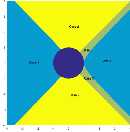
Figure 1: Illustration of the regions in the complex plane associated with the cases 1, 2 and 3 indicated in the proof of Proposition 3.5 for \theta_0 = \frac{\pi}{4} . The center circle is the unit circle.
