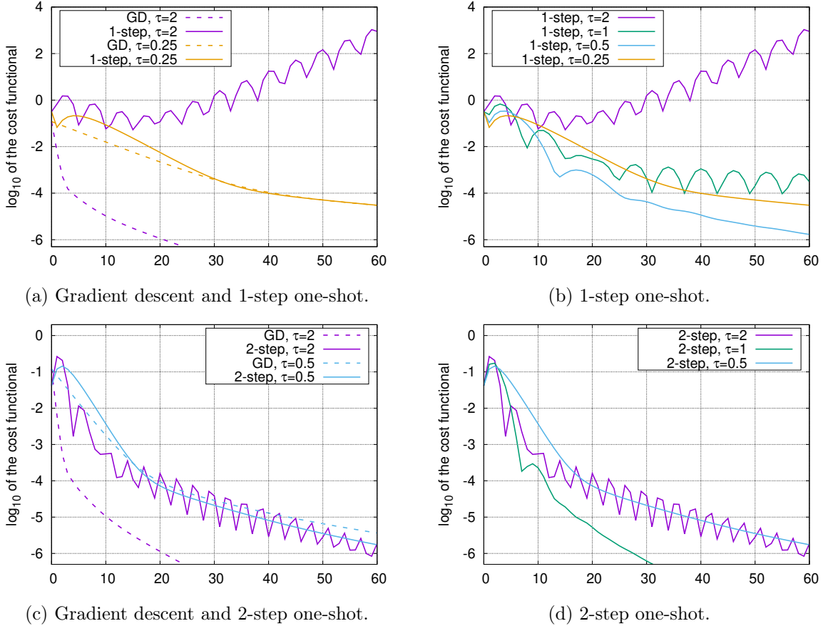
Figure 3: Convergence curves of gradient descent and k -step one-shot: dependence on the descent step \tau .
