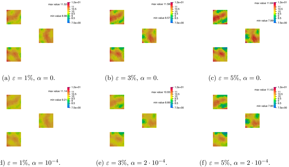
Figure 8: Reconstructed \sigma by semi-implicit 3-step one-shot with different noise levels \varepsilon . The exact \sigma is a constant function in each square with the value \sigma^{\text{ex}} = 10 .
