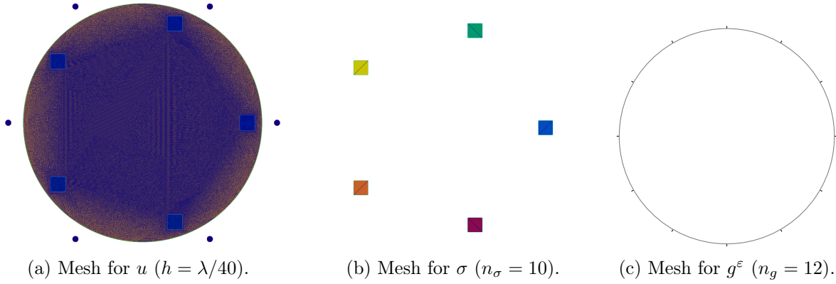
Figure 9: The configuration for the experiment of Sections 5.3 and 5.4. The values of the exact conductivity contrast is \sigma^{\text{ex}} = 10 in each square. The small circles outside the mesh for u indicate the source locations y_i , 1 \leq i \leq 6 .
