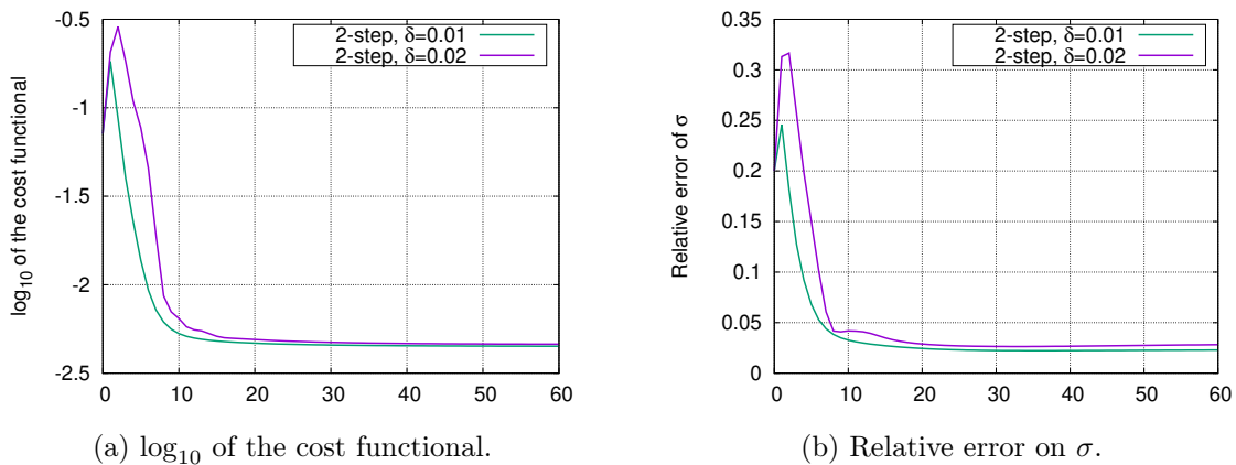
Figure 11: Result for the experiment in Section 5.4 displaying the dependence of the convergence rate for semi-implicit 2-step one-shot with respect to \delta . The descent step is \tau = 2 , the noise level is \varepsilon = 3\% and the regularization parameter is \alpha = 2 \cdot 10^{-4} .
