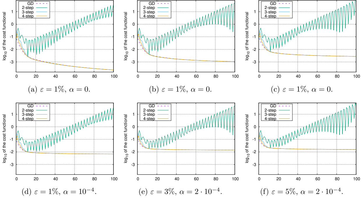
Figure 6: Convergence curves of semi-implicit gradient descent and k -step one-shot with different noise levels \varepsilon and regularization parameters \alpha . The descent step is \tau = 4.7 .
