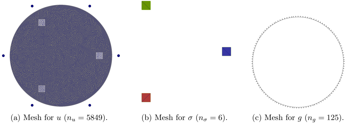
Figure 2: The configuration for the experiment in Section 5.1. The small circles outside the mesh for u indicate the source locations y_i , 1 \leq i \leq 6 .
