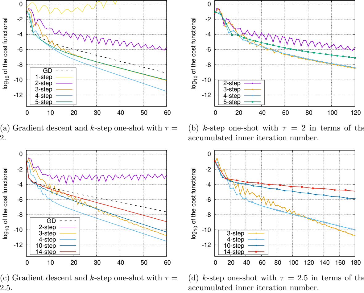
Figure 4: Convergence curves of gradient descent and k -step one-shot: dependence on the number of inner iterations k .
