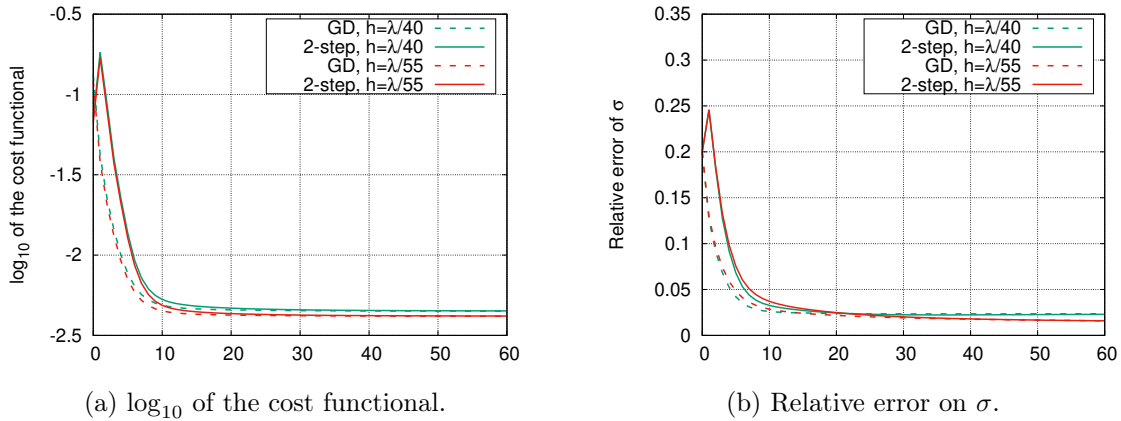
Figure 10: Result for the experiment in Section 5.3 displaying the convergence rate for semi-implicit 2-step one-shot and gradient descent with different mesh sizes for the state equations. The descent step is \tau = 2 , the noise level is \varepsilon = 3\% and the regularization parameter is \alpha = 2 \cdot 10^{-4} .
