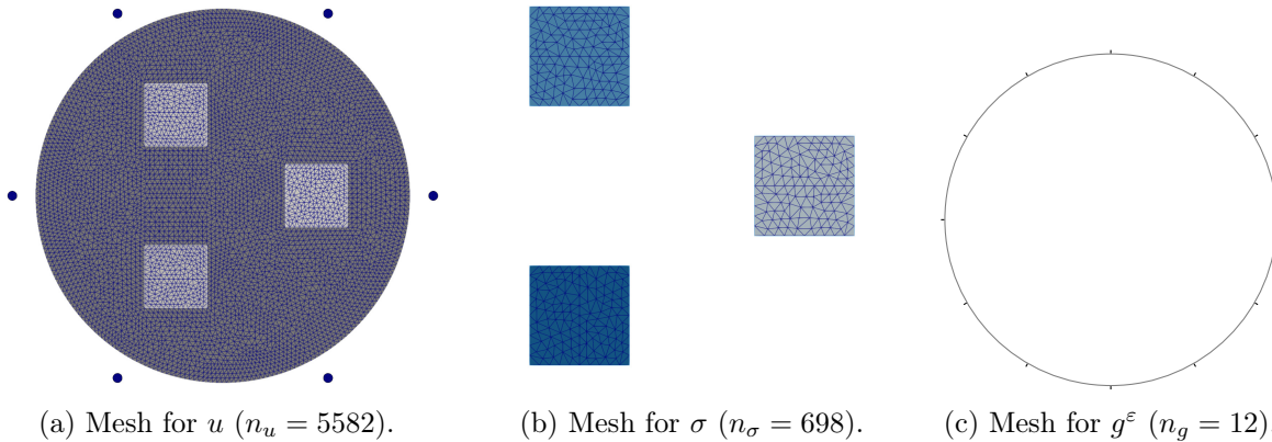
Figure 5: The configuration for the experiment in Section 5.2. The small circles outside the mesh for u indicate the source locations y_i , 1 \leq i \leq 6 .
