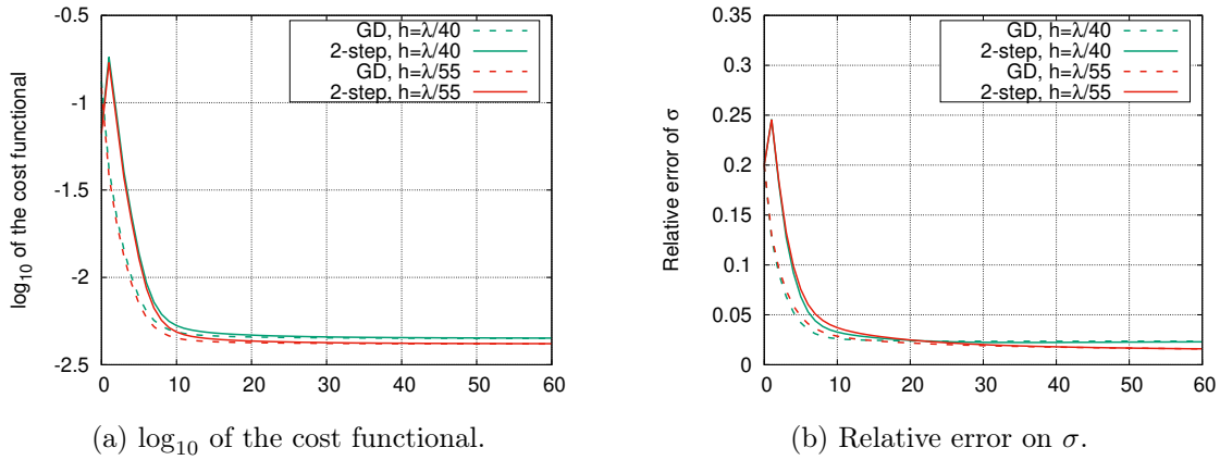
Figure 10: Result for the experiment in Section 5.3 displaying the convergence rate for semi-implicit 2-step one-shot and gradient descent with different mesh sizes for the state equations. The descent step is \tau = 2 , the noise level is \epsilon = 3\% and the regularization parameter is \alpha = 2 \cdot 10^{-4} .
