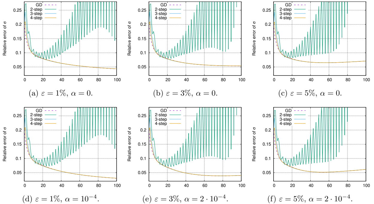
Figure 7: Convergence curves for the relative error on the parameter \sigma of semi-implicit gradient descent and k -step one-shot with different noise levels \varepsilon and regularization parameters \alpha . The descent step is \tau = 4.7 .
