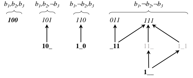
Figure 1: Minimal Accurate Subvaluations (MAS) for the Running Example. X_p - (partial)valuations corresponding to MAS are identified in bold font; X_p -valuations are in italic; X_p -partial-valuations corresponding to non-minimal accurate subvaluations are in gray; the set of benefits for which each X_p - (partial)valuation is a proof of eligibility is indicated at the top, e.g., 110 and 1_0 are eligible to benefits \{b_1 = 1, b_2 = 0, b_3 = 1\} ; X_p -valuations 000, 001, and 010 providing no benefit are not represented.
