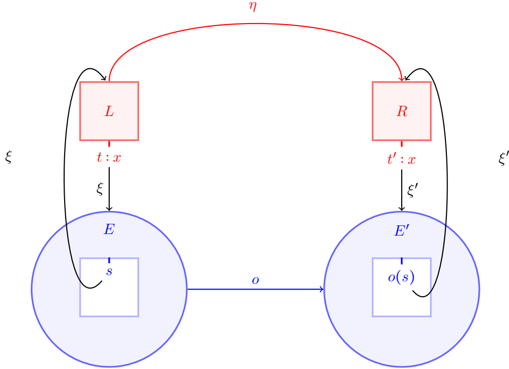
Figure 6: Compatible rewrite extension of a rewrite rule.
