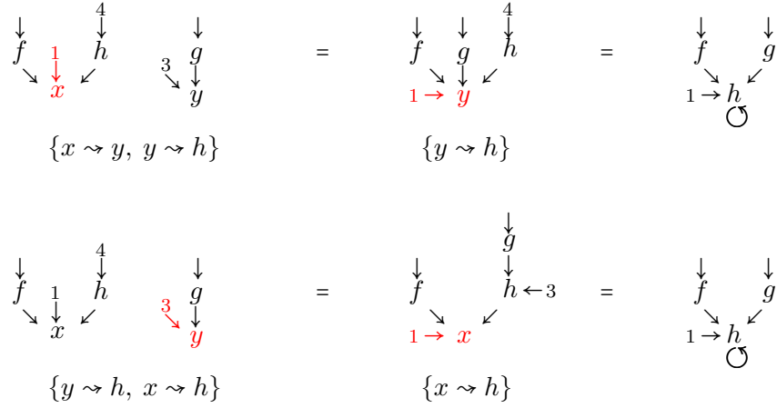
Figure 4: Formation of cycles via composition, two versions.
