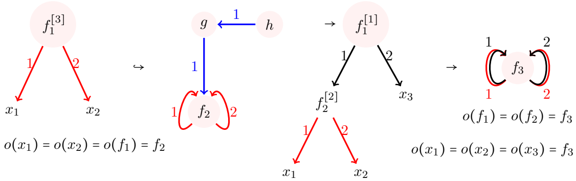
Figure 2: A monomorphism ( \rightarrow ) on the left and a morphism ( \rightarrow ) on the right. Incoming arrows at some vertex annotated with numbers stand for multiple roots.
