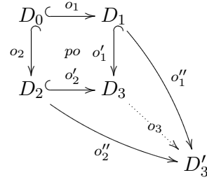
Figure 11: Pushout for drags.
