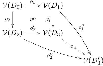
Figure 10: Pushout for sets of vertices.
