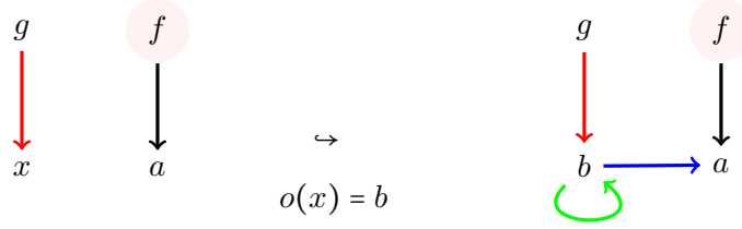
Figure 9: An injection with all four kinds of edges: black for inside, red for created, blue for entering and green for outside.
