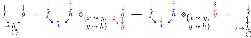
Figure 8: Rewriting with the red rule.
