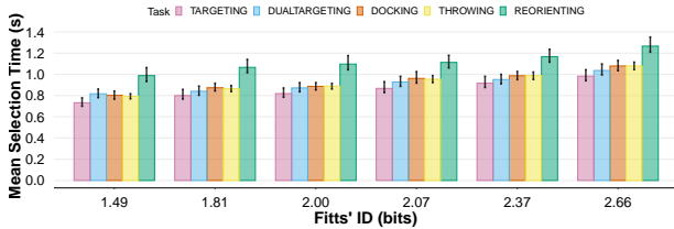
Figure 8: Mean selection time of T_{sel} by ID and Task . Error bars are shown with 95% confidence intervals.
