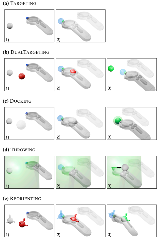
Figure 5: Illustration of visualization, selection and manipulation actions in each task. 1) Primary Target (white) appears at the left of the vanished Start Target and Secondary Target appears at the back of the Primary Target . 2) Correct selection on the Primary Target . 3) Perform the manipulation actions on either Primary Target or Secondary Target based on the task.
