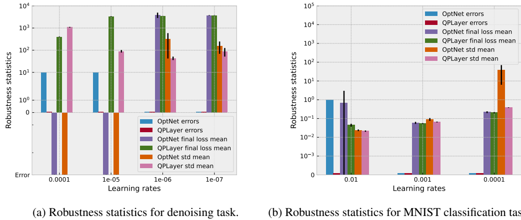
Figure 10: Robustness statistics for denoising and MNIST classification tasks: number of errors (i.e., NaNs), averaged final loss reached after 30 epochs (with 95% confidence intervals), and averaged standard deviations over the last 10 epochs (with 95% confidence intervals). Results are averaged over 10 seeds. CvxpyLayer fails to be trained for all these tasks.
