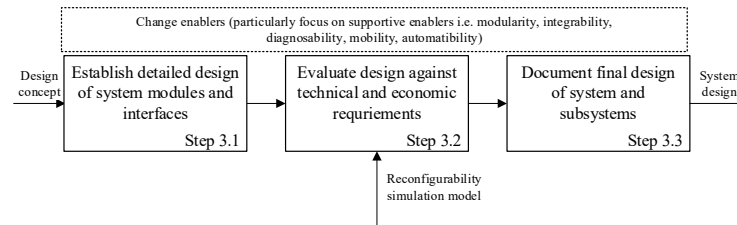
Fig. 5. Phase 3 containing detailed design of changeable system.
