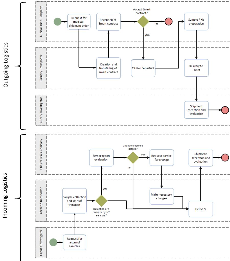
Fig. 2. Business Process Map of Reverse Logistics process for Clinical Trials integrating IoT Devices and Blockchain
