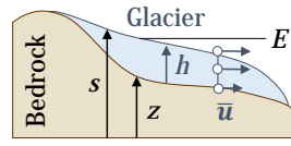
Fig. 2. Notations.
