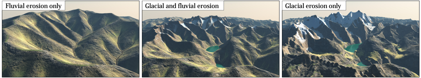
Fig. 14. While fluvial erosion on its own (left) lacks most of the main features from glacial erosion (right), it is still necessary to model the interplay between the two processes (center). Glacial erosion alone results in excessively steep cliffs, and hydraulically disconnected lakes and valleys.
