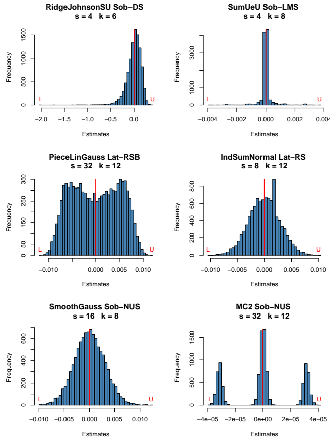
Figure 1: Some histograms of N = 10,000 integral estimates. In each case L and U mark the lower and upper extreme sample values and a red vertical line marks the integrand value 0.
