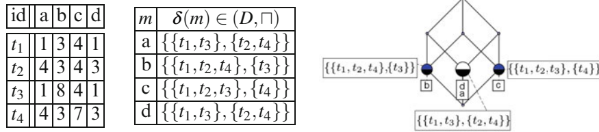
Fig. 6.2: The original data (left), the resulting pattern structure (middle) and its pattern concept lattice (right)
