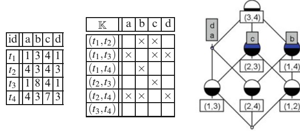
Fig. 6.1: Characterizing functional dependencies with FCA: from a set of tuples to a formal context and its concept lattice
