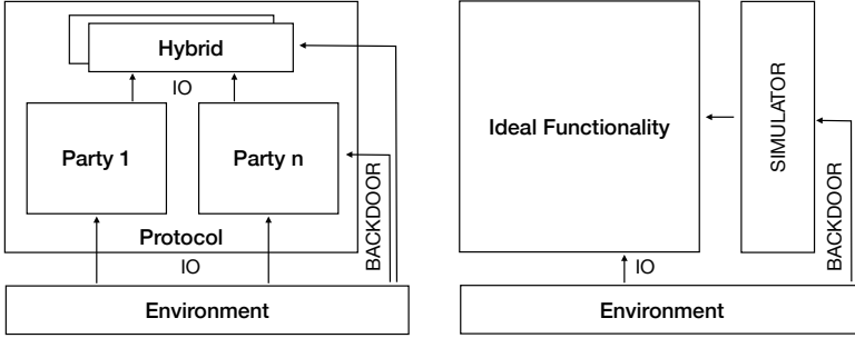
Fig. 17. Module restrictions. Arrows indicate ability to make procedure calls via the interface specified as a label; all other cross-boundary memory access is disallowed.
