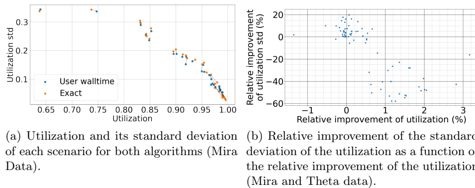
Fig. 7: Comparison of utilization and standard deviation of the utilization of EXACT and USER-WALLTIME
