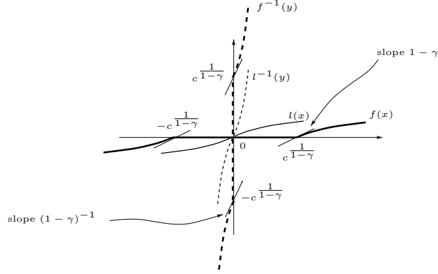
Figure 1: The functions f(\cdot) , f^{-1}(\cdot) , l(\cdot) , l^{-1}(\cdot) .
