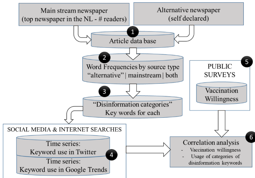
Fig. 1. Methodology overview
