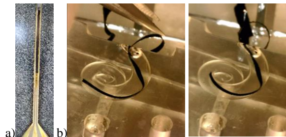
Figure 4: a) ECP-based micro-actuators clamped in a SU-8 micro-structure with integrated gold remote contacts. The actuator is a beam of 6\ \text{mm} length and 300\ \mu\text{m} wide. b) Actuation principle (without EA) inside a transparent 3D printed cochlea model. Actuator "off" on the left and "on" on the "right".
