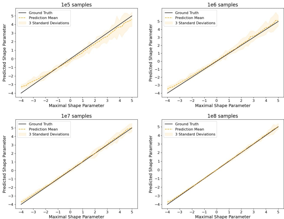
CTE via the Pickands Estimator
