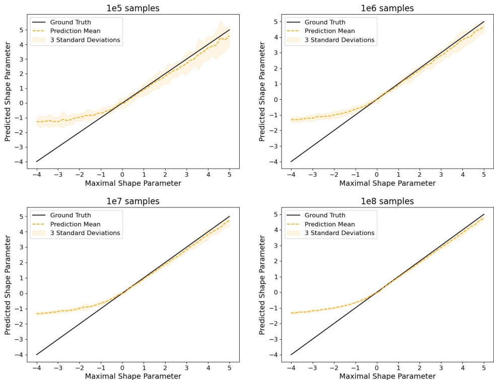
Figure 1: In cases where the maximum tail shape parameter in the mixture of conditional distributions is positive, the estimated shape parameter of the marginal is equal to this maximal value. If this maximum value is negative, the estimated shape parameter is negative. These results were obtained using the Pickands estimator.
