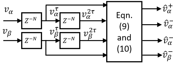
FIGURE 2 Proposed arbitrarily fast modified DSC method.
