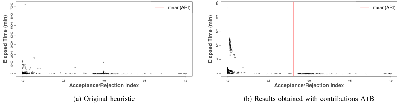
Fig. 8: Comparison of the ARI values of 722 axioms computed against DBpedia 3.9 using the original heuristic in [12] and our proposed optimization
