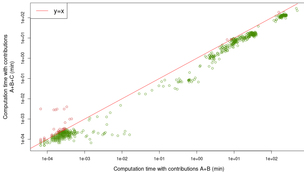
Fig. 10: Comparison of the computation times (CPU) of axioms ARIs with our first (A+B) and second (A+B+C) proposed optimizations, highlighting the proportion of axioms for which for which our last optimization saves (in green) or loose (in red) time with A+B+C. Both axes are logarithmic.
