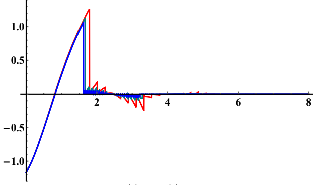
Fig. 1. Tracking Error \hat{x}_2(t) - x_2(t) Converging to 0 over Time with J Values 1 (Red), 0.5 (Green), and 0.25 (Blue) with \delta_0 = 0 and \delta_s = 0 after 4 Second Transient Period
