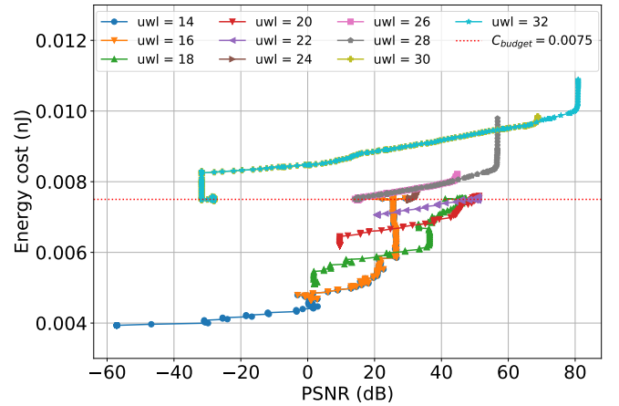
Fig. 3: Different exploration trajectories of Tabu search method corresponding to different starting points for the resource-constrained WLO problem on the FIR application. The energy budget is 0.0075 nJ. Each color corresponds to a search procedure with a given starting point. Fixed-point variables of each procedure are chosen with uniform word-lengths (UWLs) at the starting point. The number in the legend indicates the word-length given for the UWL. For each procedure, the starting point is further from the cost budget line than the ending point. Some procedures overlapped during the exploration process.
