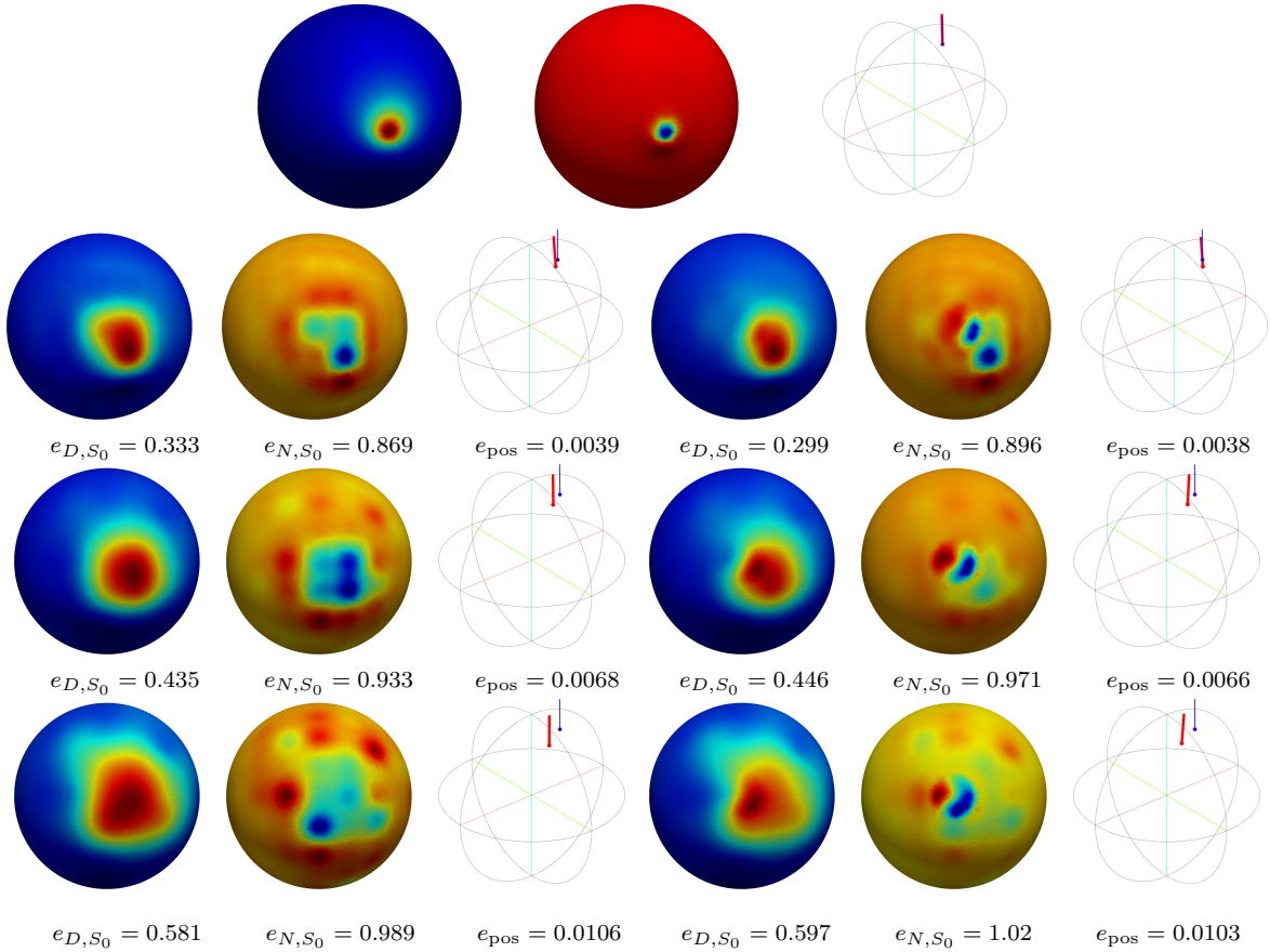
Figure 15. One close source (\mathbf{c}_{q_c}, \mathbf{p}_{q_c}) , model (b) with CSF and fontanel: QR reconstruction on the cortex with 61 electrodes and source reconstruction with FS3D. Columns 1-3: without fontanel in the QR reconstruction; Columns 4-6: taking the fontanel into account. From top to bottom: exact solution, then reconstruction with 0%, 5% and 20% noise. From left to right: Dirichlet trace, Neumann trace, source reconstruction with FS3D.
