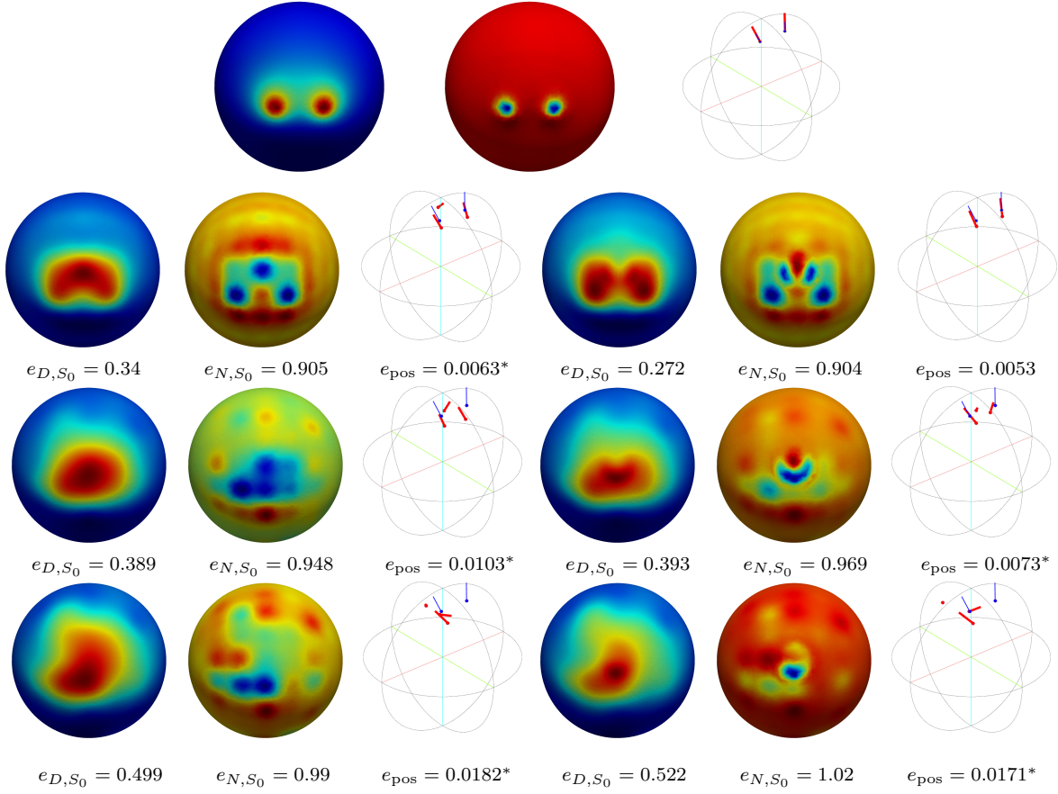
Figure 17. Two close sources ( \mathbf{c}_{q_c}, \mathbf{p}_{q_c} ) and ( \mathbf{c}_{q-c}, \mathbf{p}_{q-c} ), model (b) with CSF and fontanel: QR reconstruction on the cortex with 61 electrodes and source reconstruction with FS3D. Columns 1-3: without fontanel in the QR reconstruction; Columns 4-6: taking the fontanel into account. From top to bottom: exact solution, then reconstruction with 0%, 5% and 20% noise. From left to right: Dirichlet trace, Neumann trace, source reconstruction with FS3D. The asterisk (*) means too many reconstructed sources, and position errors with the best true/reconstructed source pairings are shown.
