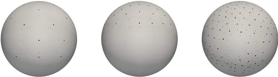
Figure 3. Electrode positions (side view). From left to right: 33, 61 and 257 electrodes test cases.
