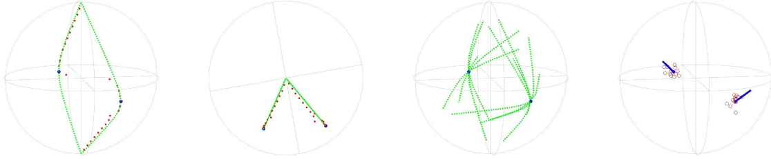
Figure 2. From left to right. (a), (b), Steps 2, 3: one direction ((0, x_3)) , Q = 2 sources (blue), theoretical singularities (green), estimated poles (red); (c), Step 3: theoretical singularity lines cross at sources locations; (d), Step 4: clustering of estimated positions (red), last least-square locations and moments tuning (blue).
