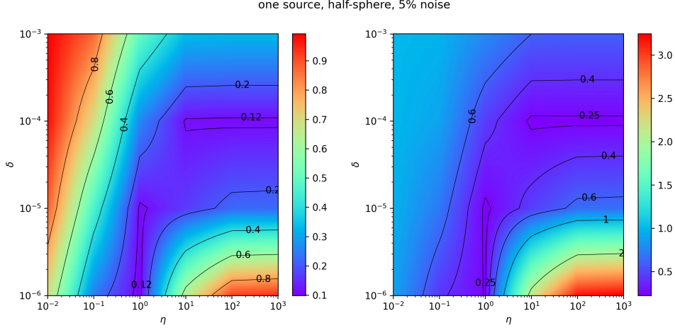
Figure 5. Relative L^2 error of the QR reconstruction in the Dirichlet (left) and Neumann (right) data at the cortex in the half sphere case with 5% noise, for varying values of \delta and \eta .
