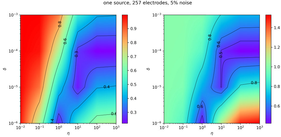
Figure 7. Relative L^2 error of the QR reconstruction in the Dirichlet (left) and Neumann (right) data at the cortex in the 257 electrodes case with 5% noise, for varying values of \delta and \eta .
