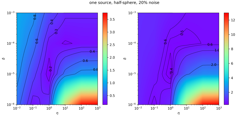
Figure 6. Relative L^2 error of the QR reconstruction in the Dirichlet (left) and Neumann (right) data at the cortex in the half sphere case with 20% noise, for varying values of \delta and \eta .
