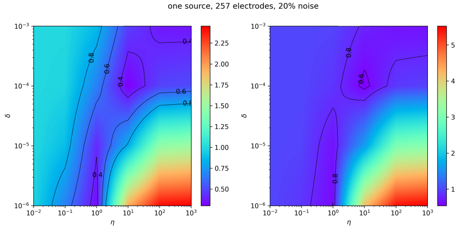
Figure 8. Relative L^2 error of the QR reconstruction in the Dirichlet (left) and Neumann (right) data at the cortex in the 257 electrodes case with 20% noise, for varying values of \delta and \eta .
