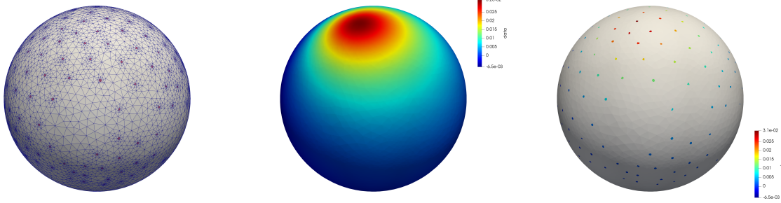
Figure 4. From left to right: mesh adapted to the electrode patches, exact synthetic data on scalp, average value of the potential on each electrode patch used as input data for QR.
