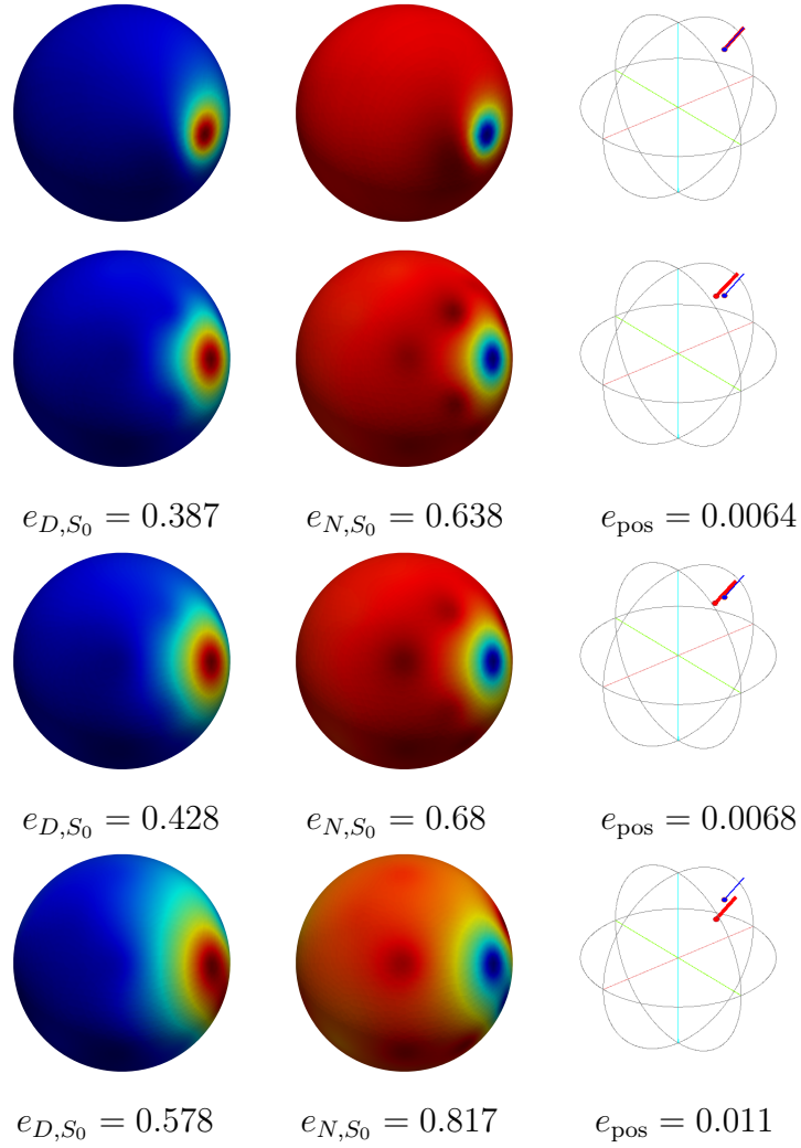
Figure 9. One distant source (\mathbf{c}_{q_d}, \mathbf{p}_{q_d}) and head model (a): QR reconstruction on the cortex with 33 electrodes and source reconstruction with FS3D. From top to bottom: exact solution, then reconstruction with 0%, 5% and 20% noise. From left to right: Dirichlet trace, Neumann trace, source reconstruction with FS3D.
