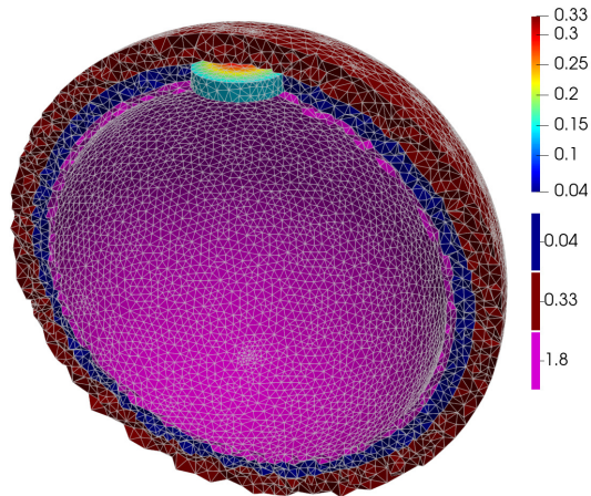
Figure 14. Mesh of the three conductivity regions around the cortex corresponding to CSF, skull and scalp, including the main fontanel region with varying conductivity.
