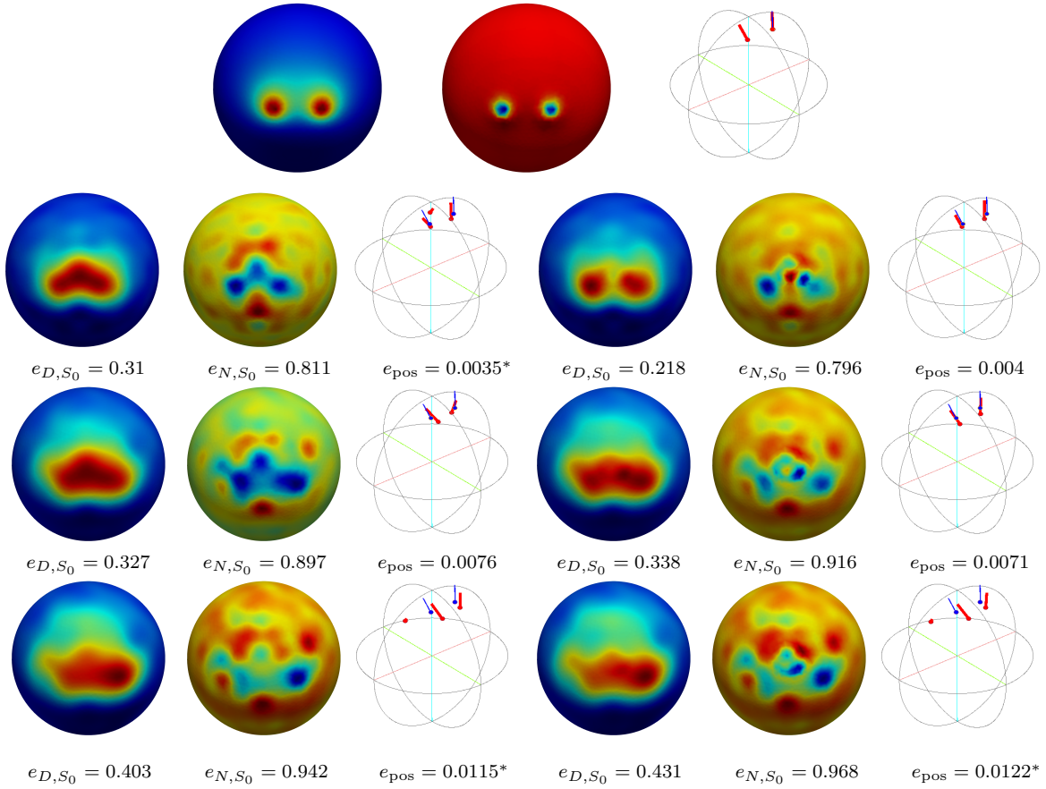
Figure 18. Two close sources ( \mathbf{c}_{q_c}, \mathbf{p}_{q_c} ) and ( \mathbf{c}_{q-c}, \mathbf{p}_{q-c} ), model (b) with CSF and fontanel: QR reconstruction on the cortex with 257 electrodes and source reconstruction with FS3D. Columns 1-3: without fontanel in the QR reconstruction; Columns 4-6: taking the fontanel into account. From top to bottom: exact solution, then reconstruction with 0%, 5% and 20% noise. From left to right: Dirichlet trace, Neumann trace, source reconstruction with FS3D. The asterisk (*) means too many reconstructed sources, and position errors with the best true/reconstructed source pairings are shown.
