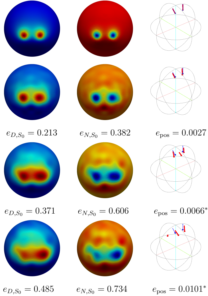
Figure 13. Two close sources (\mathbf{c}_{q_c}, \mathbf{p}_{q_c}) and (\mathbf{c}_{q_{-c}}, \mathbf{p}_{q_{-c}}) and head model (a): QR reconstruction on the cortex with 257 electrodes and source reconstruction with FS3D. From top to bottom: exact solution, then reconstruction with 0%, 5% and 20% noise. From left to right: Dirichlet trace, Neumann trace, source reconstruction with FS3D. The asterisk (*) means too many reconstructed sources, and position errors with the best true/reconstructed source pairings are shown.
