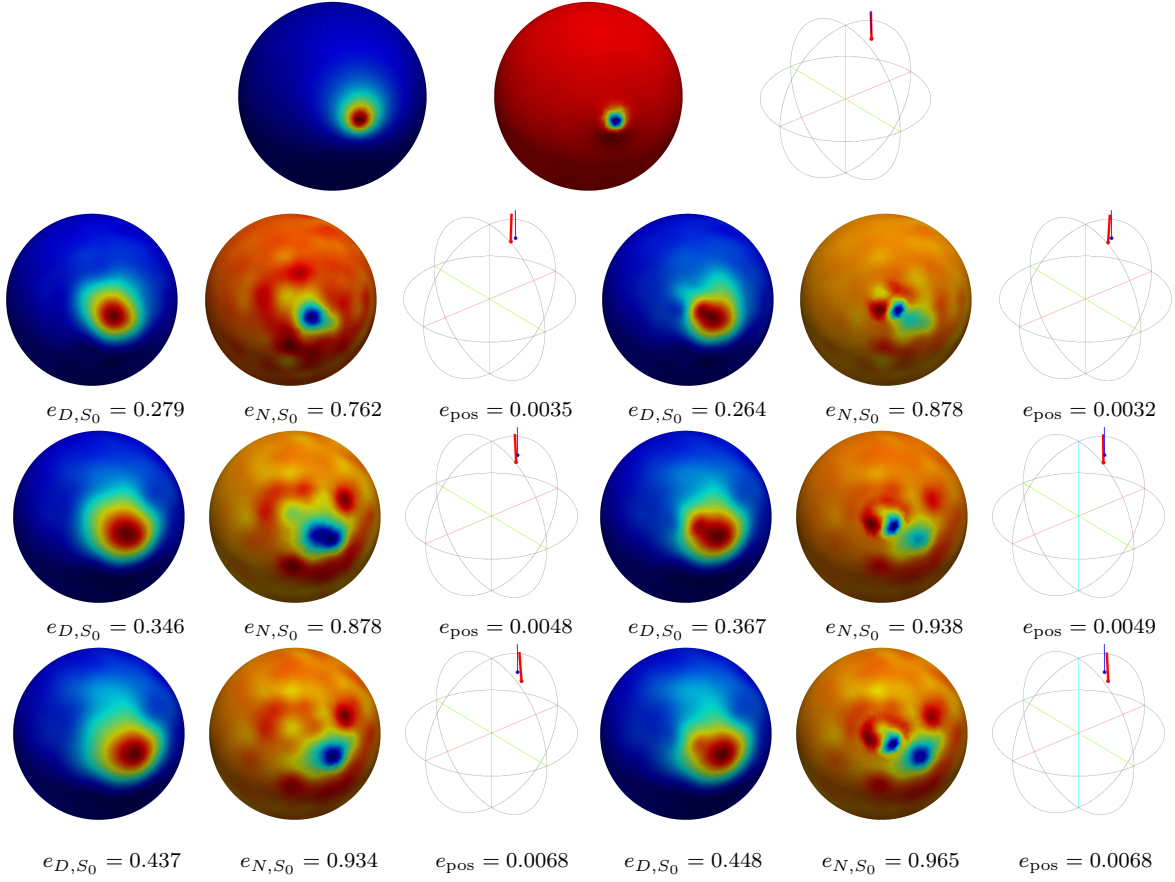
Figure 16. One close source (\mathbf{c}_{q_c}, \mathbf{p}_{q_c}) , model (b) with CSF and fontanel: QR reconstruction on the cortex with 257 electrodes and source reconstruction with FS3D. Columns 1-3: without fontanel in the QR reconstruction; Columns 4-6: taking the fontanel into account. From top to bottom: exact solution, then reconstruction with 0%, 5% and 20% noise. From left to right: Dirichlet trace, Neumann trace, source reconstruction with FS3D.
