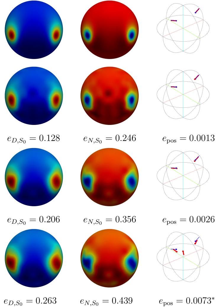
Figure 12. Two distant sources (\mathbf{c}_{q_d}, \mathbf{p}_{q_d}) and (\mathbf{c}_{q-d}, \mathbf{p}_{q-d}) , head model (a): QR reconstruction on the cortex with 257 electrodes and source reconstruction with FS3D. From top to bottom: exact solution, then reconstruction with 0%, 5% and 20% noise. From left to right: Dirichlet trace, Neumann trace, source reconstruction with FS3D. The asterisk (*) means too many reconstructed sources, and position error with the best true/reconstructed source pairing is shown.
