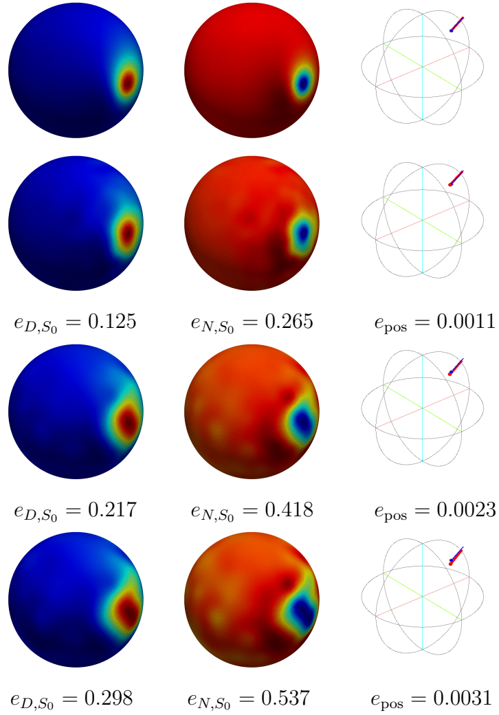
Figure 11. One distant source ( \mathbf{c}_{q_d}, \mathbf{p}_{q_d} ) and head model (a): QR reconstruction on the cortex with 257 electrodes and source reconstruction with FS3D. From top to bottom: exact solution, then reconstruction with 0%, 5% and 20% noise. From left to right: Dirichlet trace, Neumann trace, source reconstruction with FS3D.
