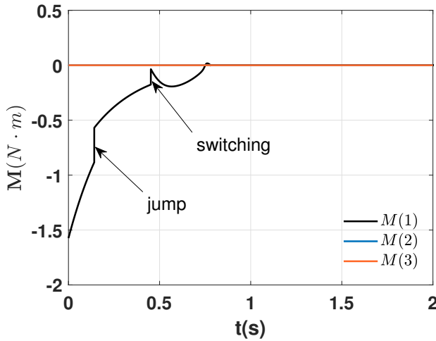
Fig. 3. Control input M
