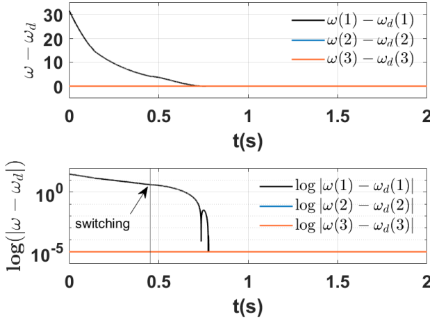
Fig. 2. Angular velocity error \omega_d - \omega
