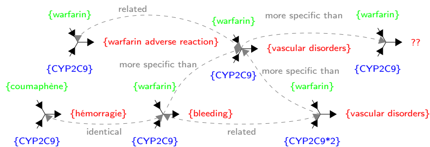
Fig. 2. Example of heterogeneity issues and expected matching results (dashed gray arrows) between PGx tuples. The phenotype is unknown (denoted ??) for one tuple, coumaphène and hémorragie are the French words for warfarin and hemorrhage, which in turn is a synonym of bleeding. CYP2C9*2 is a gene variant that is more specific than the gene CYP2C9 itself, bleeding is more specific than vascular disorder according to an ontology, and vascular disorders is related somehow to warfarin adverse reaction.
