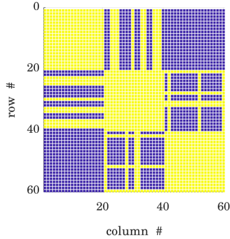
Fig. 2: Color map for the connectivity matrix of the tensegrity-like structure, generated using proposed method; blue correspond to no connection, yellow to a connection
