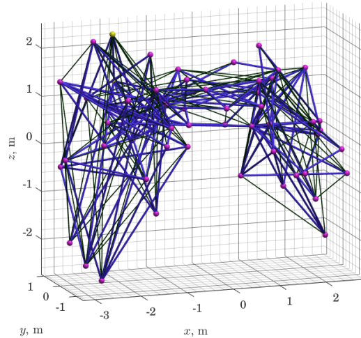
Fig. 1: Example of a tensegrity-like structure, generated using proposed method; the nodes are shown in purple, cables are shown in black and struts are shown in blue
