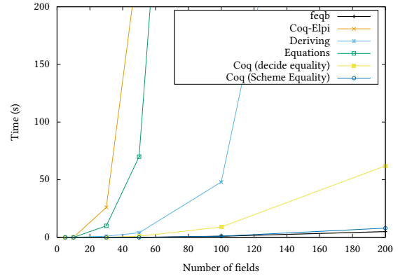
(b) On records
