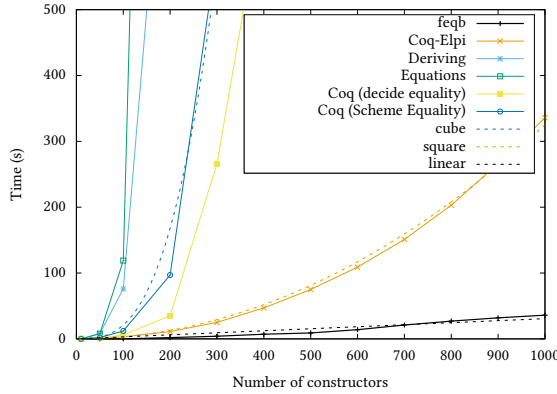
(a) On flat inductive types
