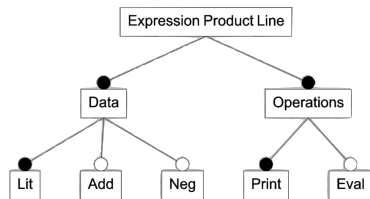
Figure 2: Feature Model for Expression Problem Product Line
