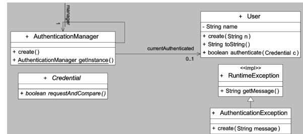
Figure 6: Design Class Diagram for the Authentication Base
