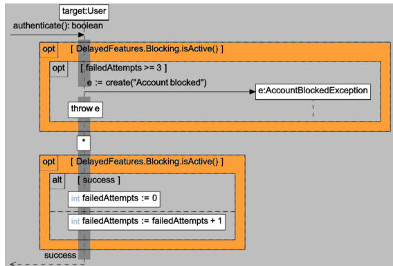
Figure 12: Blocking behavior with Toggz Check
