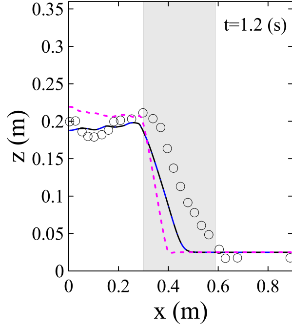
Figure 7: water surface elevation in glass bead case: dashed line: ( \alpha_l = 3000 , \alpha_t = 3 ); solid line ( \alpha_l = 3000 , \alpha_t = 0.1 ); dash-dotted line: ( \alpha_l = 600 , \alpha_t = 3 ); blank circle: experimental data
