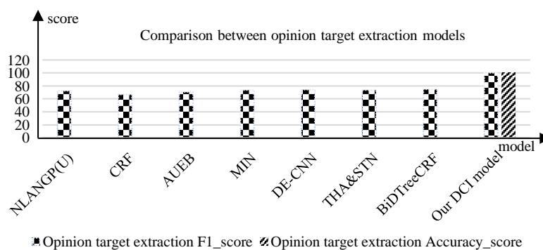
Figure 4. F1, accuracy of previous models and our deep CNN-IOB2 model in opinion target extraction
