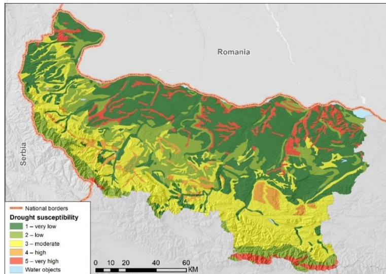
Fig. 5. Drought susceptibility according to the soil types
