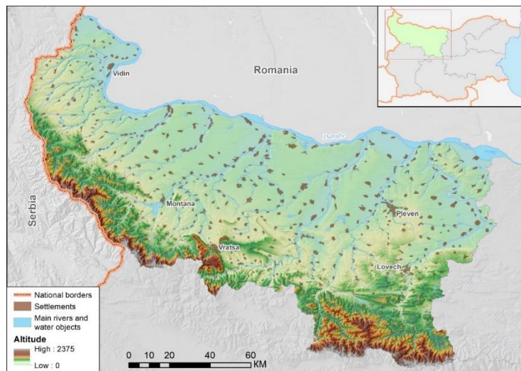
Fig. 1. Study area – NUTS 2 region Severozapad
