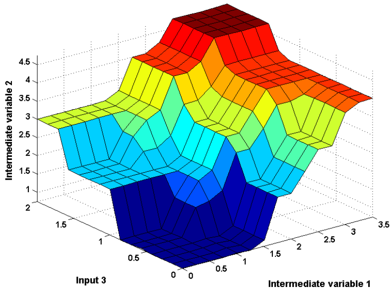
Fig. 7. Inference surfaces of the Fuzzy logic subsystem 2
