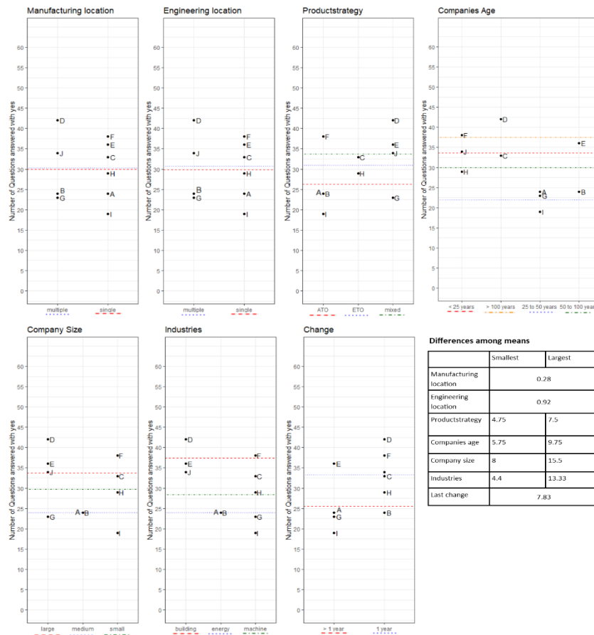
Fig. 4. Factorwise analysis
