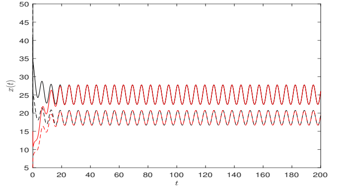
Fig. 2. The state trajectories versus the time t for LV model
