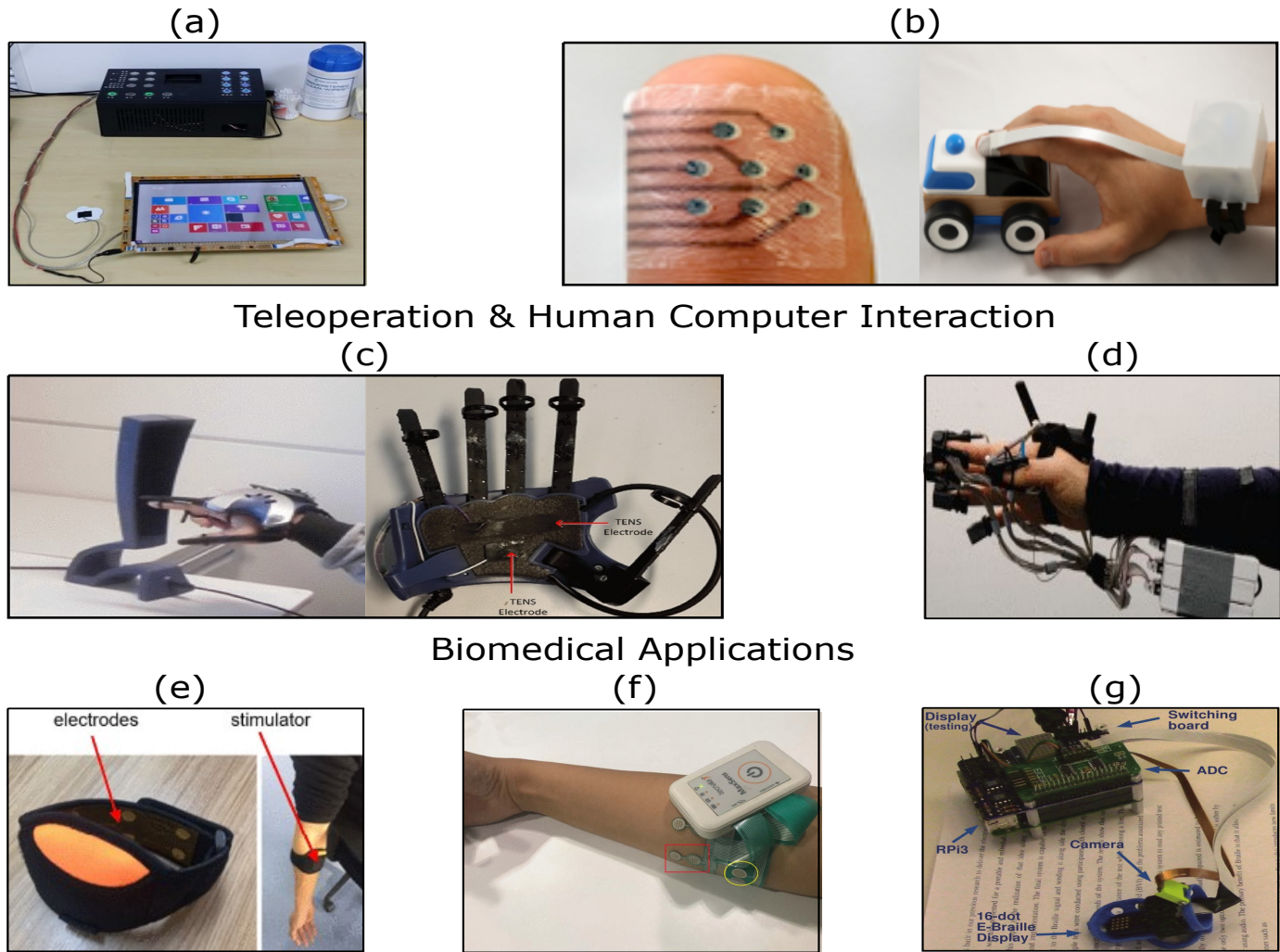
Fig. 4. Representative examples of electro-tactile feedback systems per implementation: (a) transparent touchpad [26]; (b) thin epidermal electrodes for augmented haptics [28]; (c) glove for dorsal hand stimulation [24]; (d) multi-finger stimulation [123]; (e) armband for prosthetics [111]; (f) armband for prosthetics [91]; (g) braille reading system [127].
