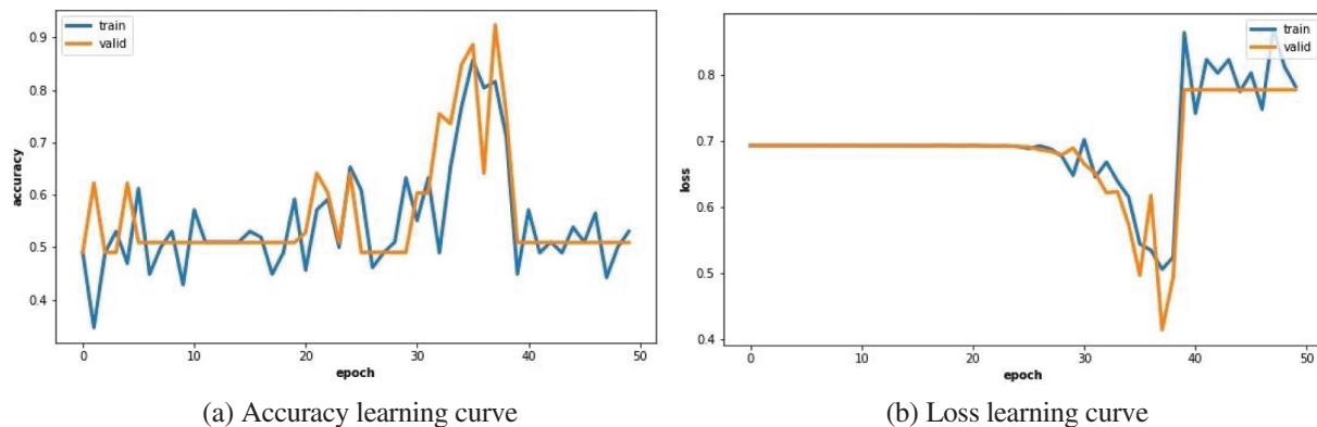
Figure 5: Learning curves on dataset B without using pre-trained weights
