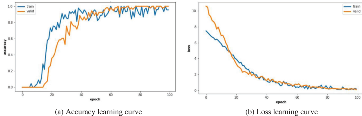
Figure 7: Learning curves on dataset A without using pre-trained weights with the train (blue) and validation (orange) data: (a) accuracy vs. epoch and (b) loss vs. epoch
