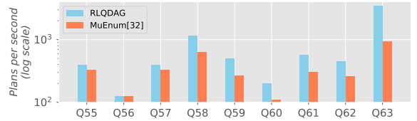
Figure 20: Non-regular queries.
