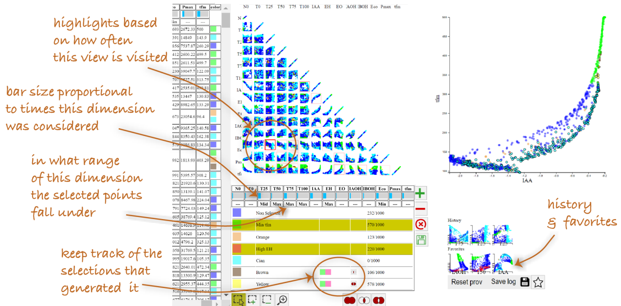
Fig. 1. The VisProm technology probe includes several in-visualization provenance views to aid trade-off analysis.
