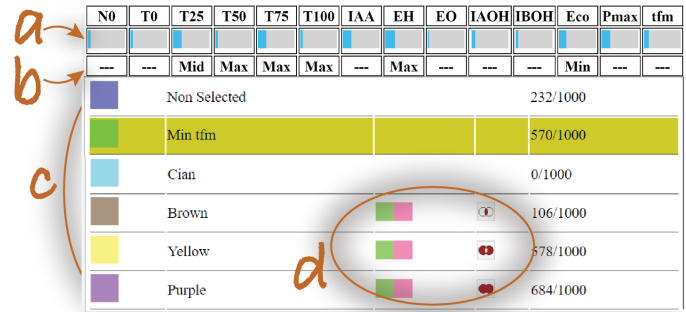
Fig. 3. The query selection panel includes: the dimension names and their DimensionCounts (a) as a bar that is filled depending on frequency; the SelectionRange tool (b) that indicates with text in what range (if any) the current selection falls under for the particular dimension; and finally (c) all queries/selections. Selections can be renamed (like the active selection Min tfm ) and their colors changed. For selections that were created by group operations between other selections, their SelectionOrigin (original selections and operation) can be seen next to their name (d).
