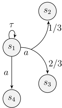
(a) A NPLTS N
