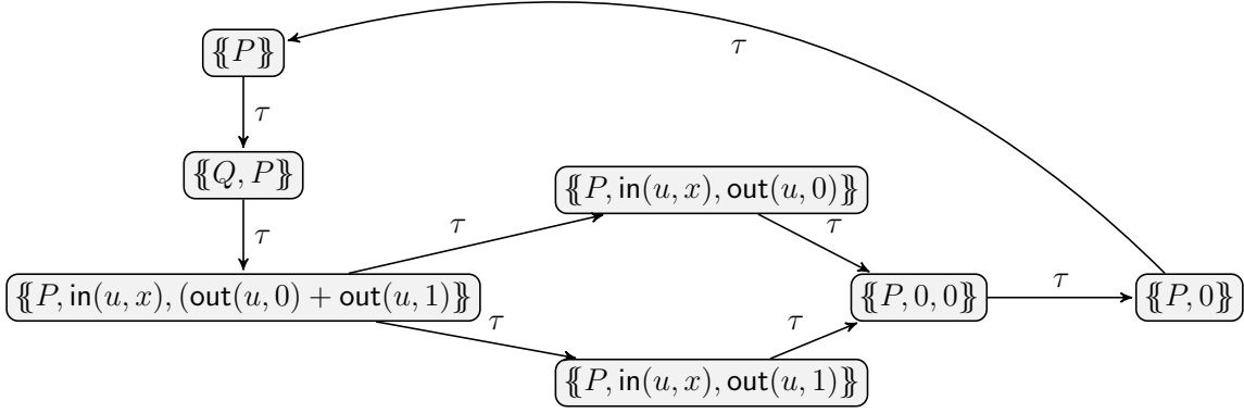
Figure 4: A cycle in \mathbf{N}^o , from Example 2
