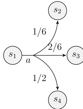
(c) A randomized resolution for N \text{corr}(s_i) = s_i ( 1 \leq i \leq 3 )
