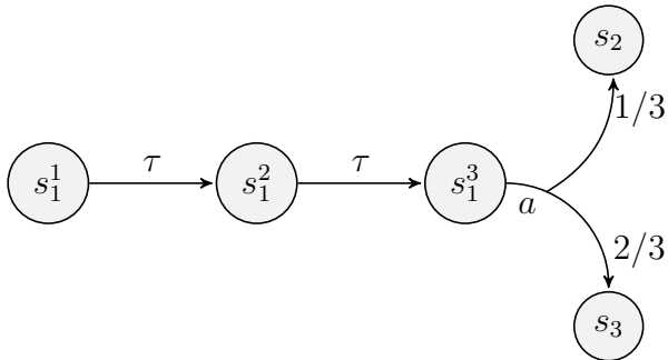
(b) A non-randomized resolution for N \text{corr}(s_1^i) = s_1 ( 1 \leq i \leq 3 ), \text{corr}(s_j) = s_j ( 2 \leq j \leq 3 ).
